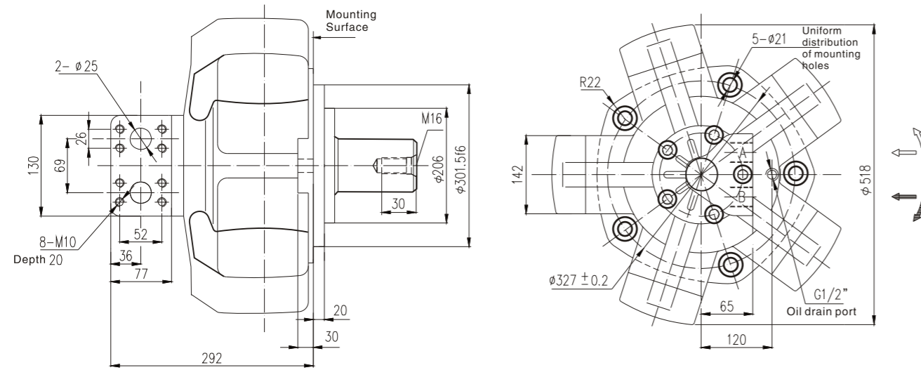
Standard outside spline NHM16-**
