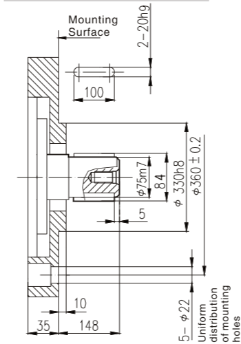
Standard outside spline NHM16-** D
