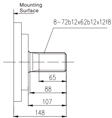
Standard outside spline NHM16-**
