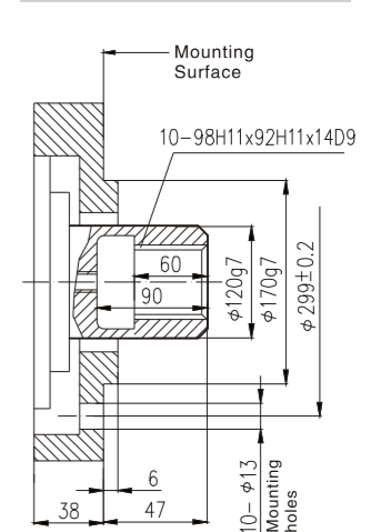
Standard inside spline NHM16-** I 32
